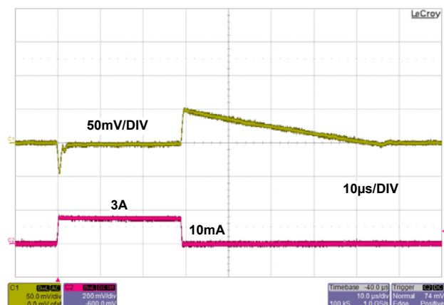
FIGURE 11. LOAD TRANSIENCE FOR V_{OUT} = 1.8V , C_{OUT} = 22\mu F , C_{pb} = 82pF
