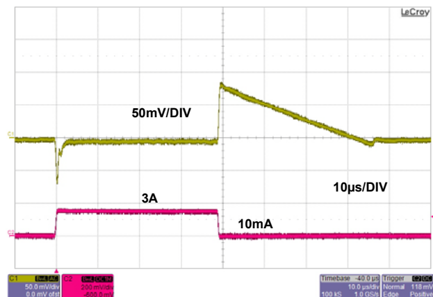
FIGURE 13. LOAD TRANSIENCE FOR V_{OUT} = 2.5V , C_{OUT} = 10\mu F , C_{pb} = 47pF
