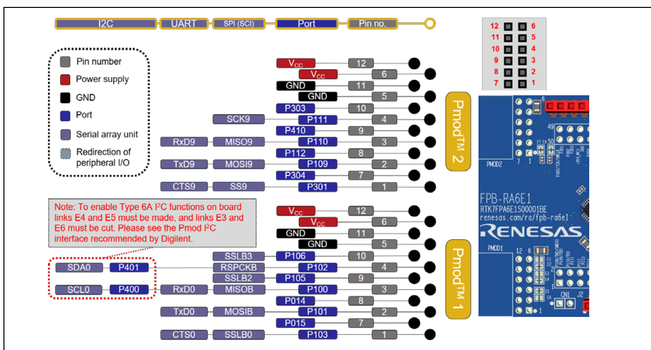
Figure 3. FPB-RA6E1 Pmod Interface
