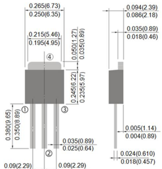
TO-251AA Dimension
