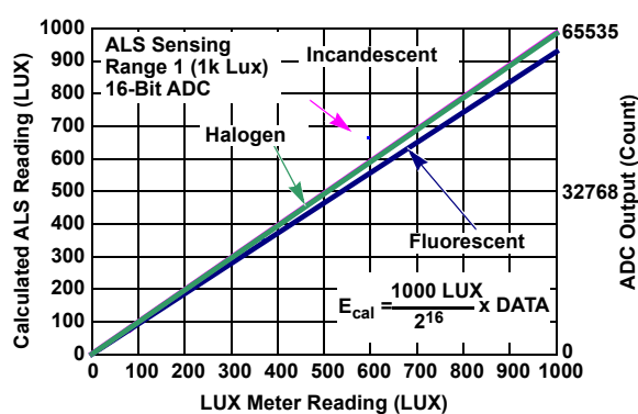
Figure 31. Indicated lux vs Actual
