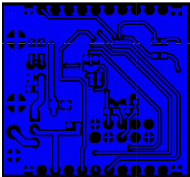
Figure 29. Bottom Layer, USB Daughter Board
