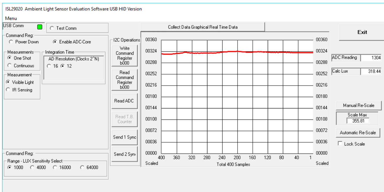
Figure 15. Static GUI
