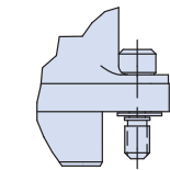
Code H Socket Head Jackscrew
