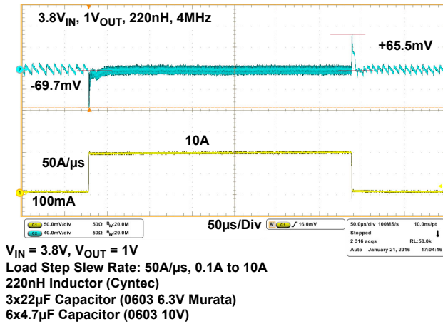
Figure 17. Dual-Phase Load Transient (10A/200ns)
