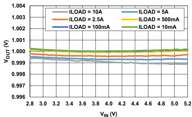
Figure 27. Dual-Phase, V_{OUT} vs V_{IN} (10mA to 10A)
