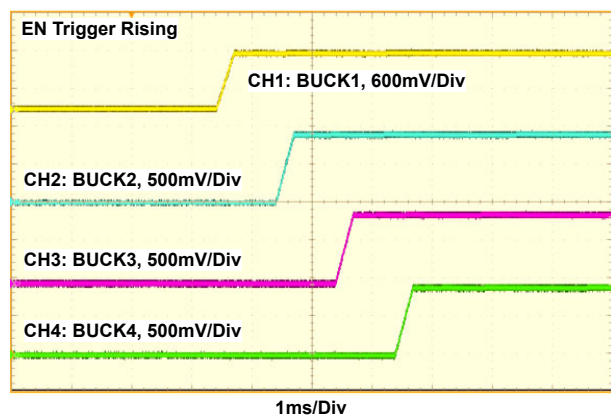
Figure 25. ISL91212B Startup by EN, V_{OUT1, 2, 3, 4} = 0.9V
