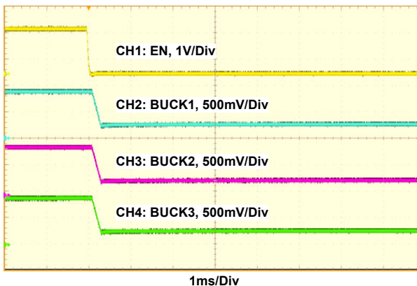
Figure 24. ISL91212A Shutdown by EN, V_{OUT1, 2, 3} = 0.9V
