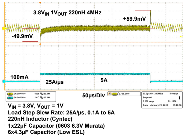
Figure 18. Single-Phase Transient (5A/200ns)
