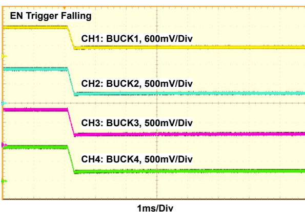
Figure 26. ISL91212B Shutdown by EN, V_{OUT1, 2, 3, 4} = 0.9V
