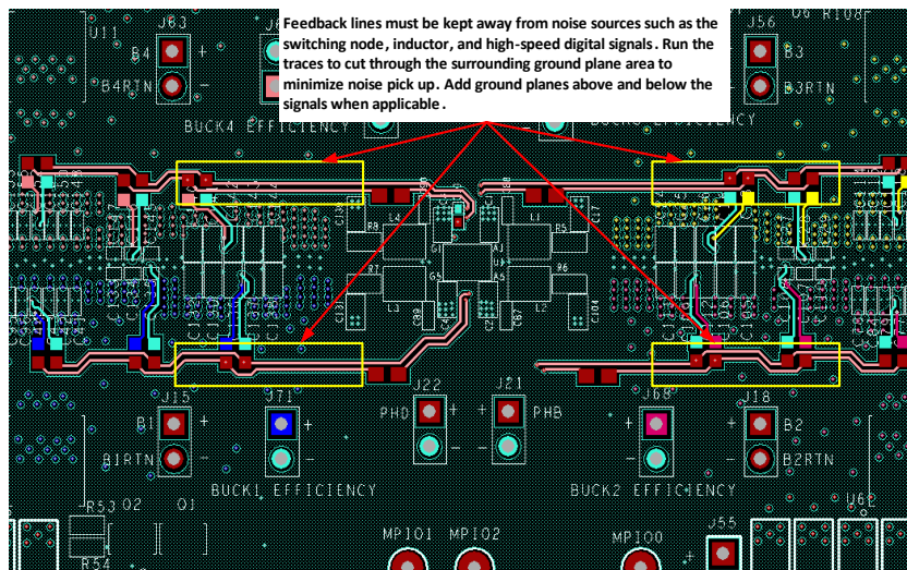
Figure 47. Recommended PCB Layout Bottom Layer
