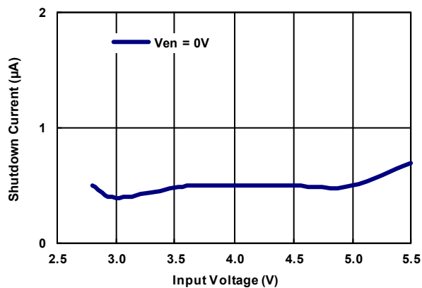
Figure 32. Shutdown Current vs V_{IN}
