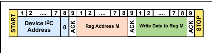
Figure 40. 1 Byte Write to Register M
