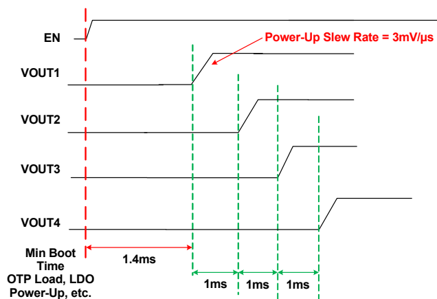
Figure 36. Chip Power-Up Example
