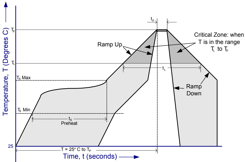
Figure 9-5 FT120 Solder Reflow Profile
