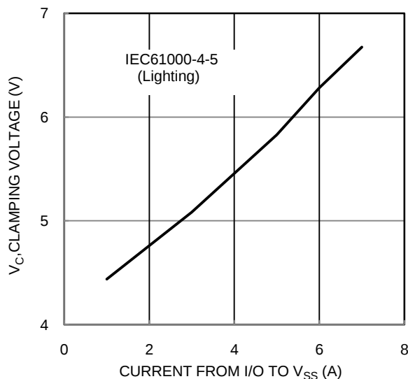
Figure 6 Clamping Voltage Characteristic
