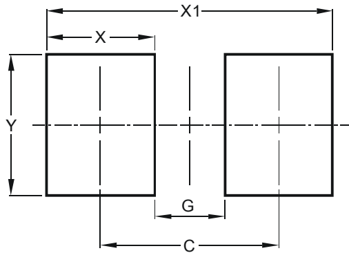
X1-DFN1006-2
