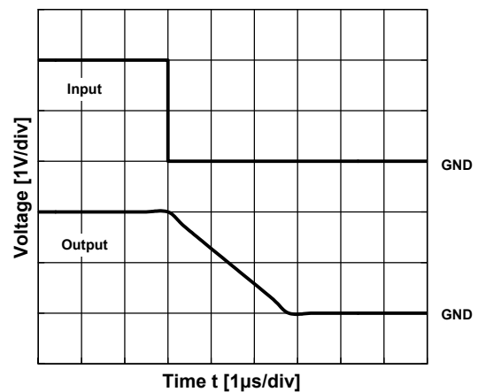
Pulse Response (Fall)
