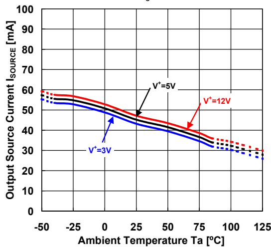
Output Source Current vs. Temperature (Supply Voltage) V_O = 0\text{V}
