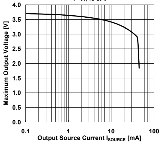
Maximum Output Voltage vs. Output Source Current V^- = 5\text{V} , T_a = 25^\circ\text{C}
