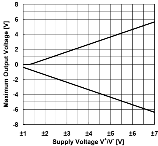
Maximum Output Voltage vs. Supply Voltage R_L = \infty , T_a = 25^\circ\text{C}
