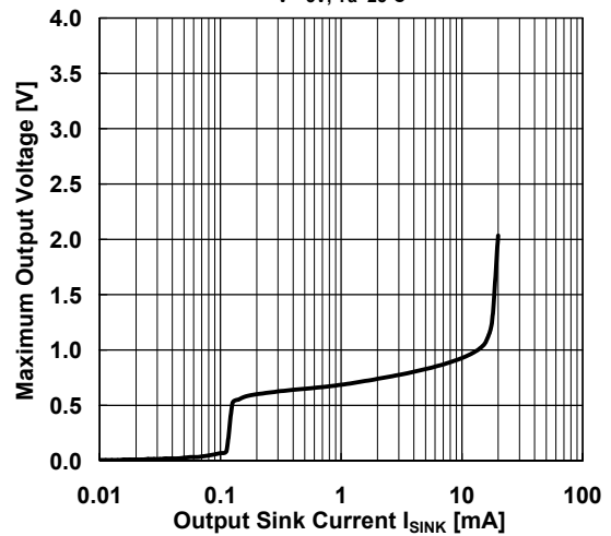
Maximum Output Voltage vs. Output Sink Current V^- = 5\text{V} , T_a = 25^\circ\text{C}
