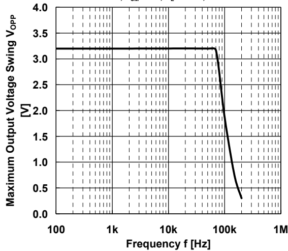
Maximum Output Voltage Swing vs. Frequency
