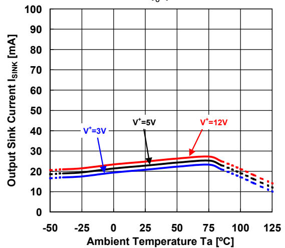
Output Sink Current vs. Temperature (Supply Voltage) V_O = V^+
