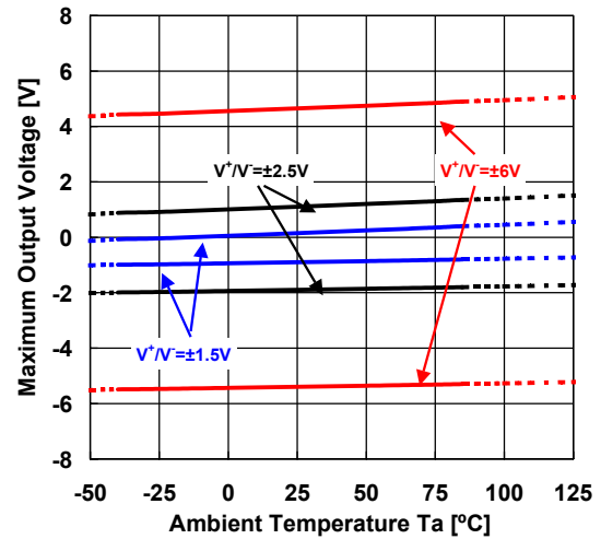
Maximum Output Voltage vs. Temperature (Supply Voltage) R_L = \infty
