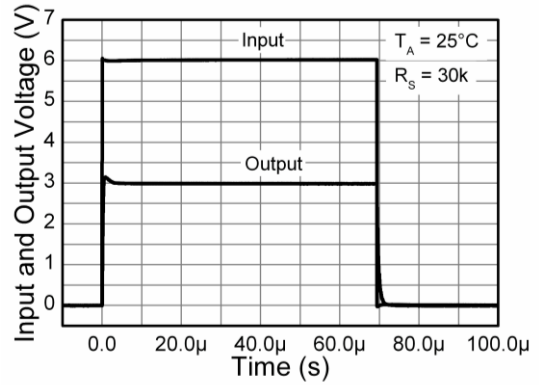
Long Pulse Response LM4040-30Q
