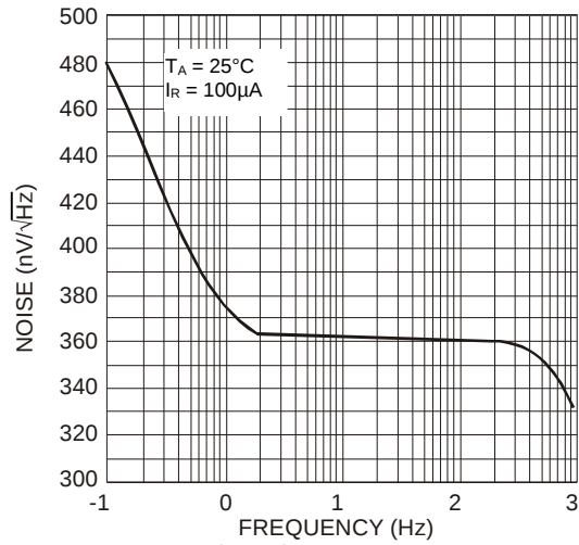
Noise Voltage vs. Frequency LM4040-25Q
