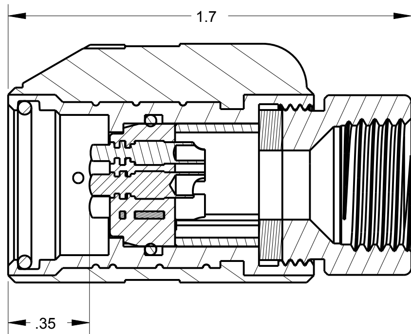
SECTION Z-Z SCALE 2.500
