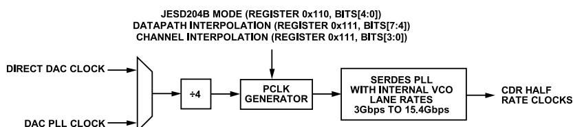
Figure 28. SERDES PLL Synthesizer Block Diagram Including VCO Divider Block
