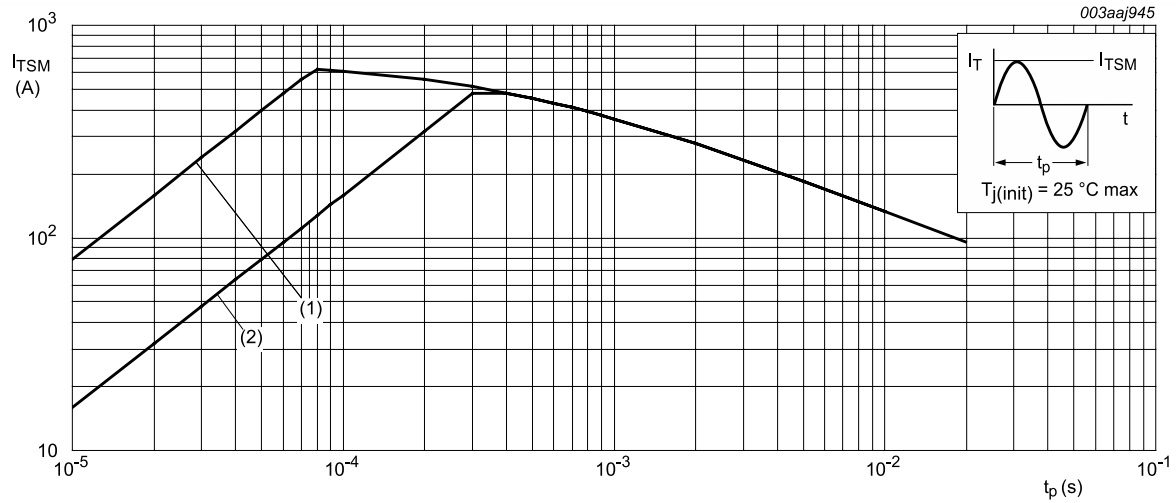
t_p \leq 20\text{ ms} (1) dI_T/dt limit (2) T2- G+ quadrant limit Fig. 5. Non-repetitive peak on-state current as a function of pulse width; maximum values
