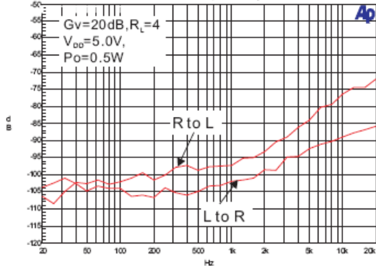
9. Crosstalk VS Frequency
