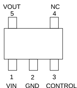
SMV(SOT-25)(SC-74A)
