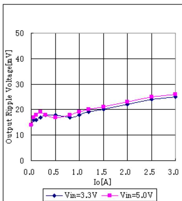
Fig.9-1-9. Ripple Voltage v. s. Output Current
