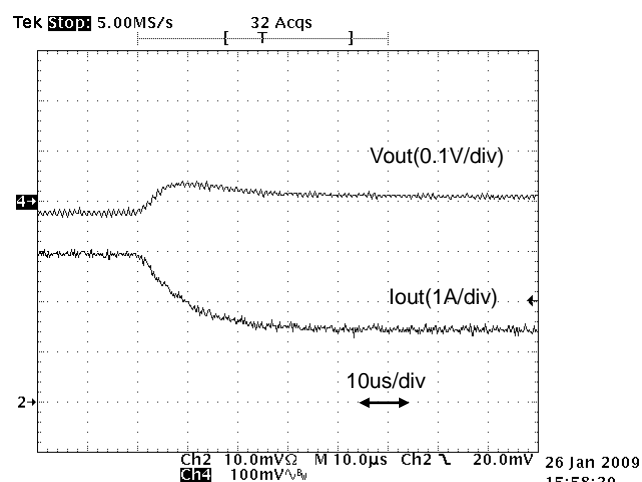
Fig.9-2-4. Load Transient Response ( I_o=3\rightarrow1.5A )
