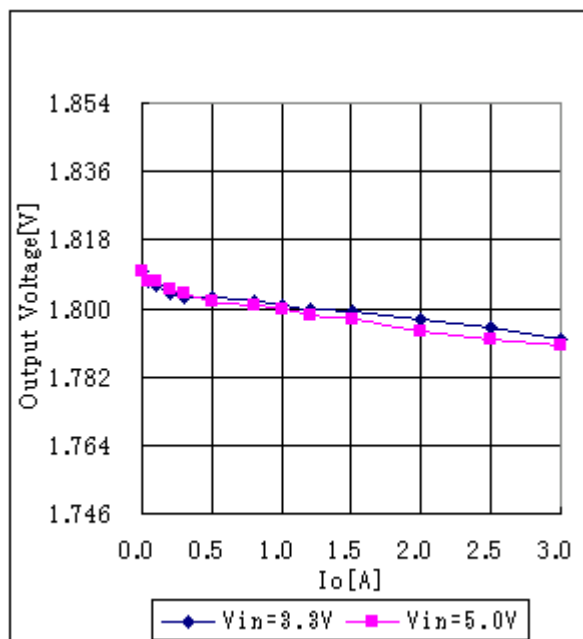
Fig.9-1-7. Output Voltage v.s. Output Current
