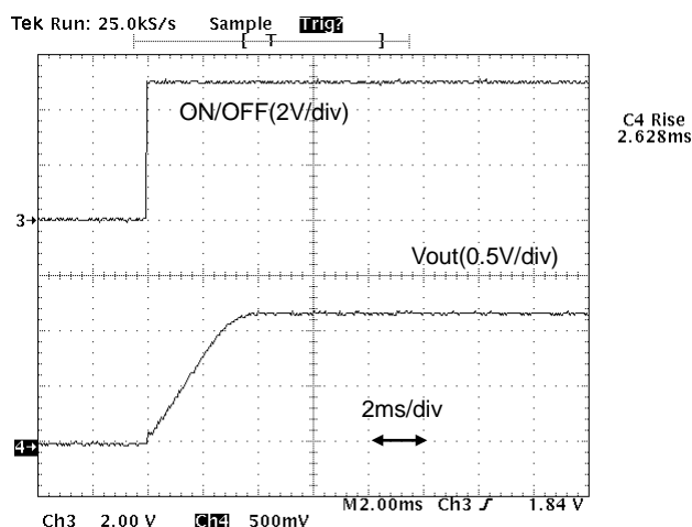
Fig.9-2-5. Start-up Waveform ( I_o=0A )
