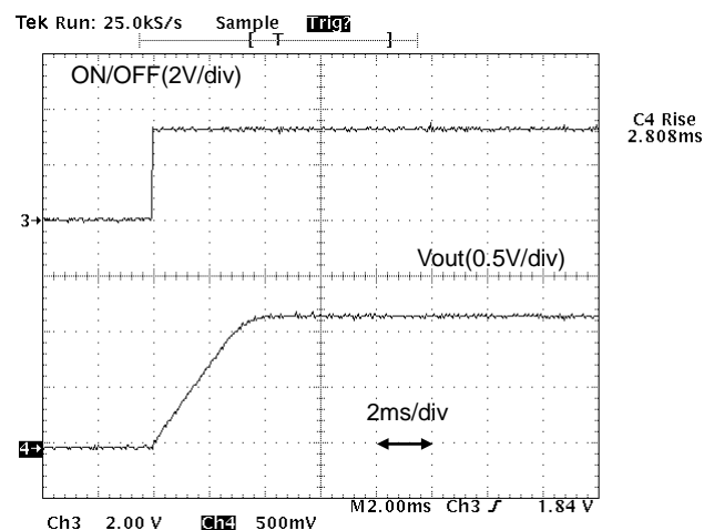
Fig.9-2-2. Start-up Waveform ( I_o=3A )
