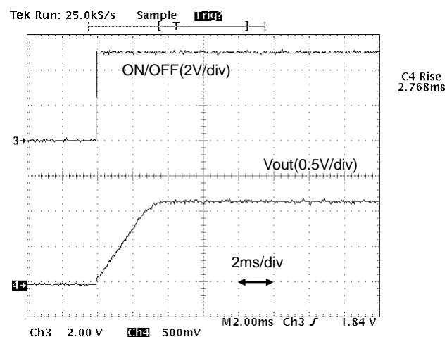
Fig.9-2-6. Start-up Waveform ( I_o=3A )
