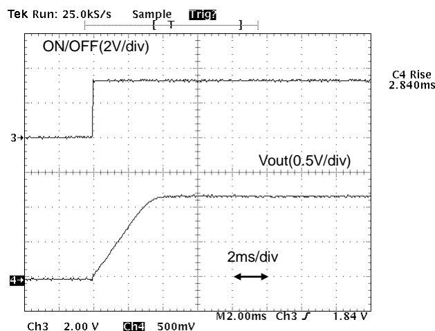
Fig.9-2-1. Start-up Waveform ( I_o=0A )
