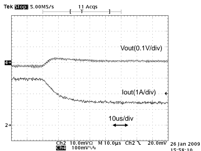
Fig.9-2-8. Load Transient Response (I_o=3 \rightarrow 1.5A)
