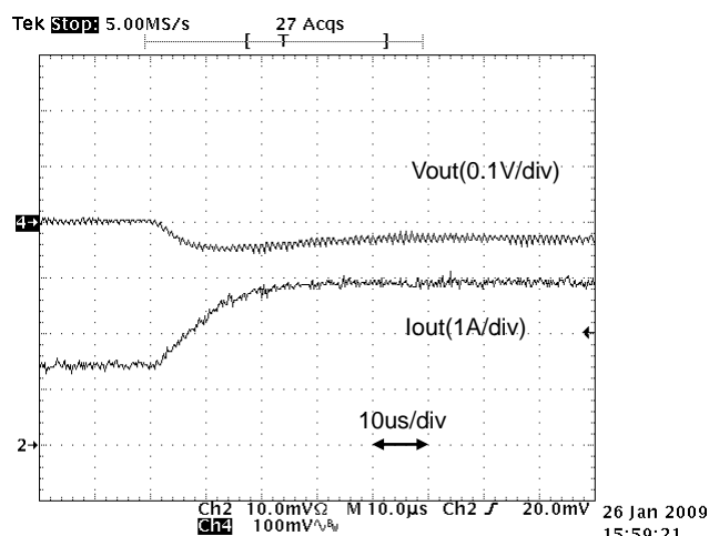
Fig.9-2-7. Load Transient Response (I_o=1.5 \rightarrow 3A)
