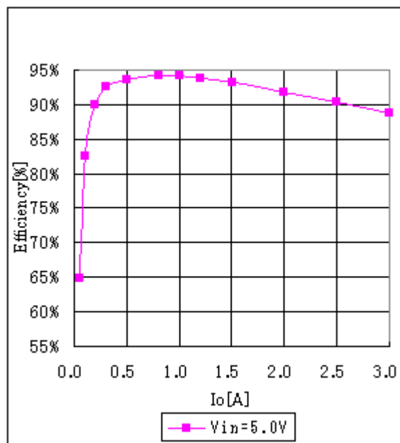
Fig.9-1-11. Efficiency v.s. Output Current
