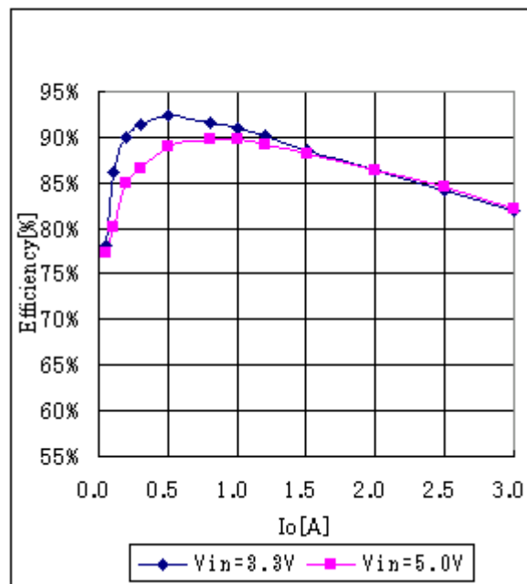
Fig.9-1-8. Efficiency v.s. Output Current
