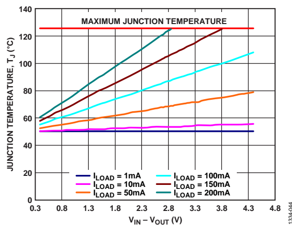
Figure 46. TSOT, 500 mm 2 of PCB Copper, T_A = 50^\circ\text{C}
