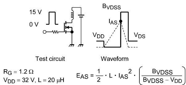
Fig. 8.15 Test Circuit/Waveform
