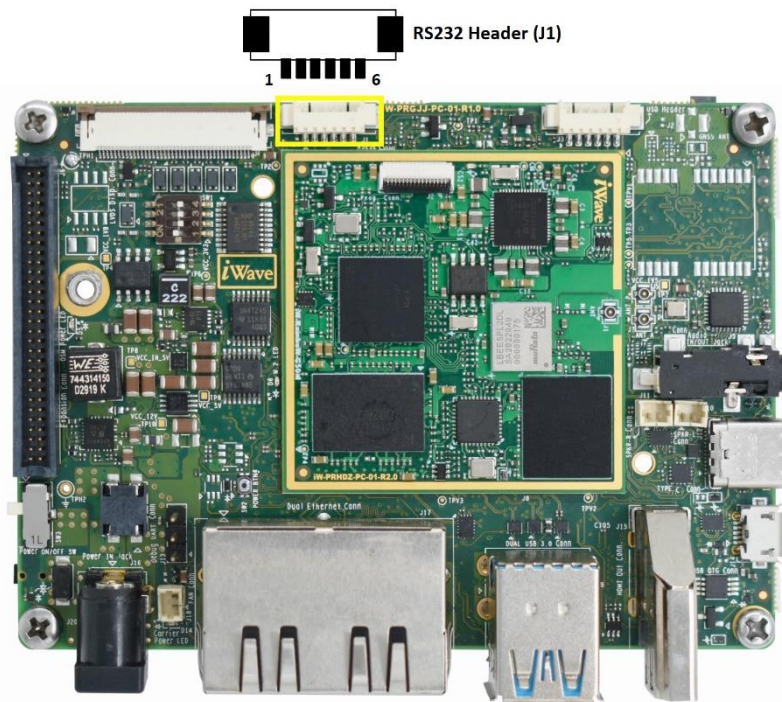
Figure 15: RS232 Header
