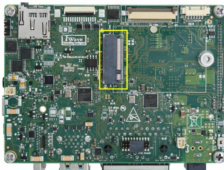
Figure 23: M.2 Key B Connector
