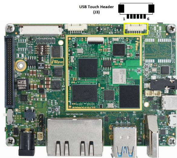
Figure 18: USB Touch Connector
