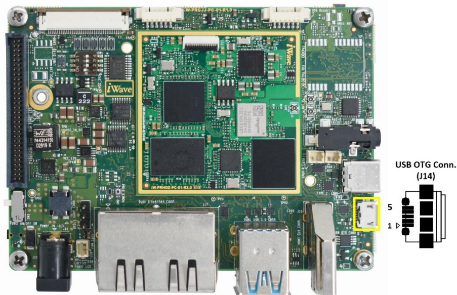
Figure 8: USB OTG Connector
