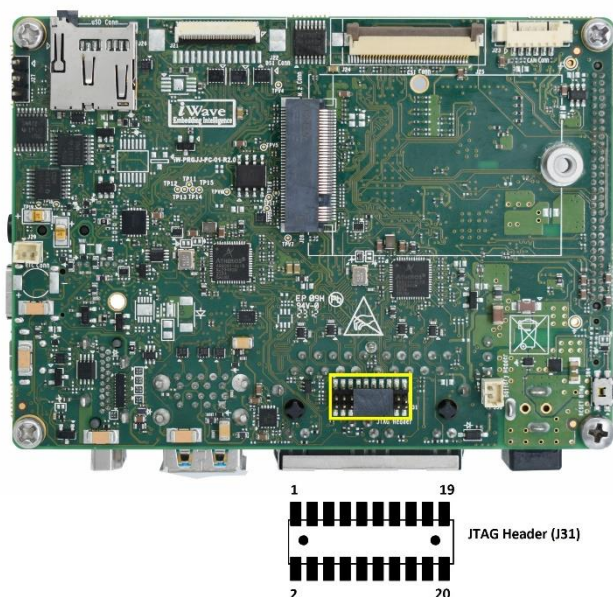
Figure 28: JTAG Header
