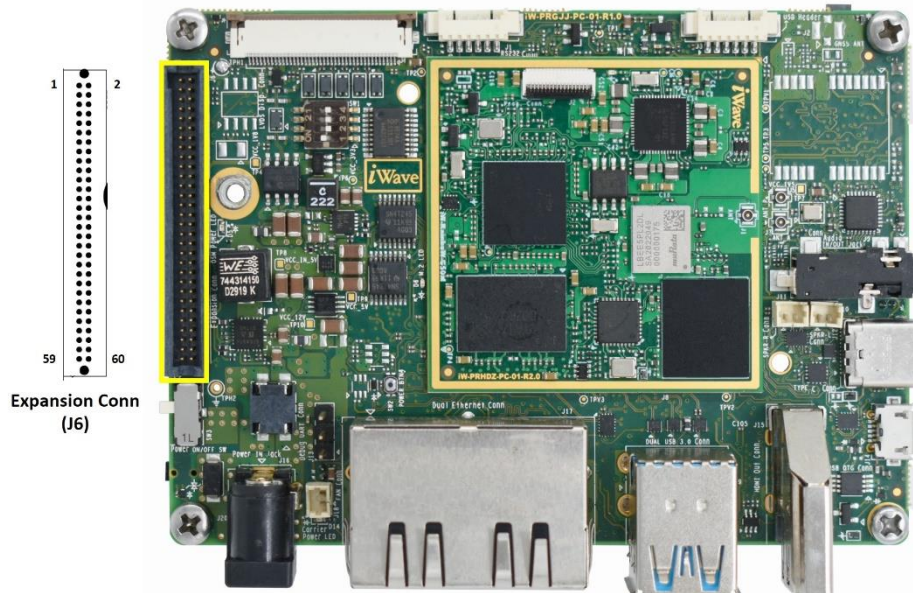
Figure 25: Expansion Connector
