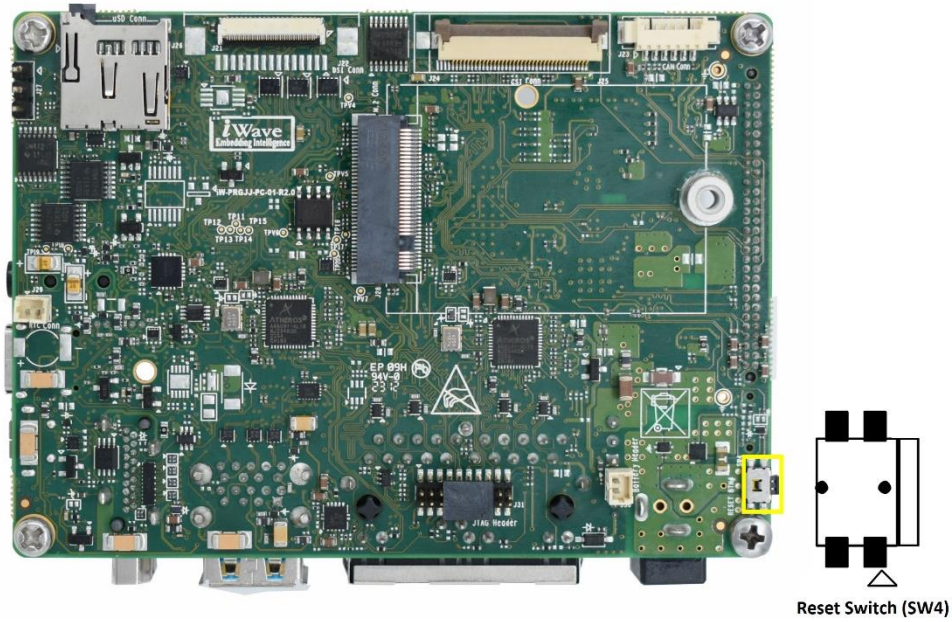
Figure 30: Reset Switch
