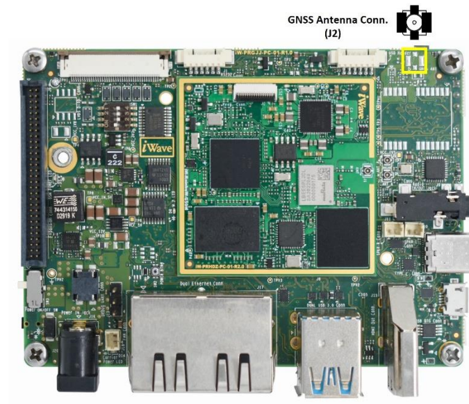
Figure 10: GNSS Antenna Connector
