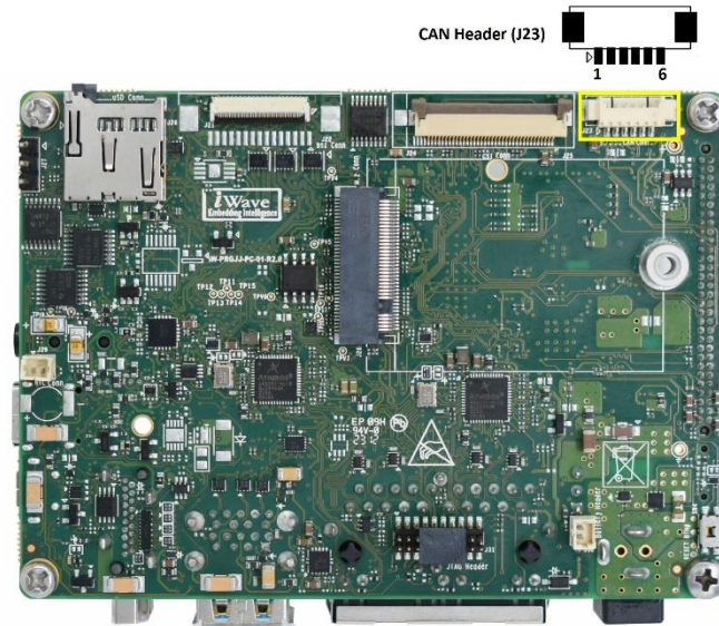
Figure 13: CAN Header
