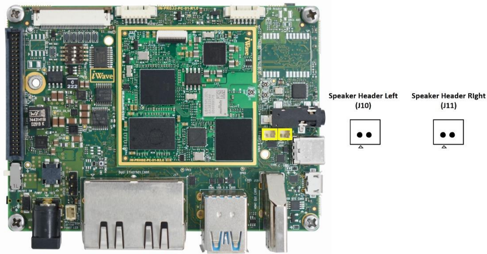
Figure 22: Speaker Headers
