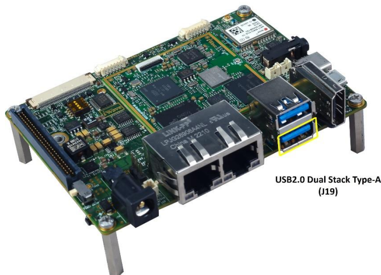
Figure 12: USB2.0 Host-Bottom Port
