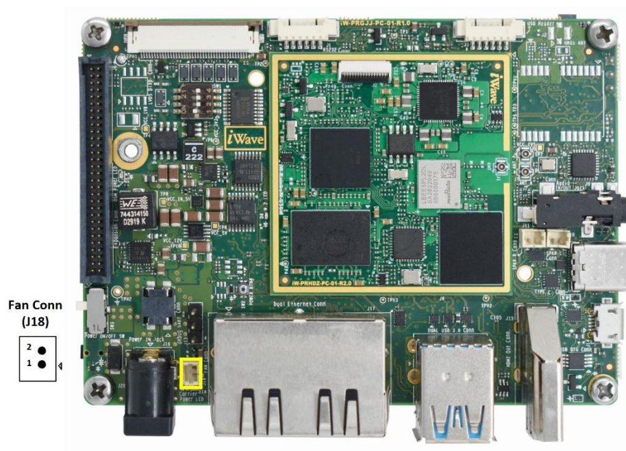
Figure 26: Fan Connector
