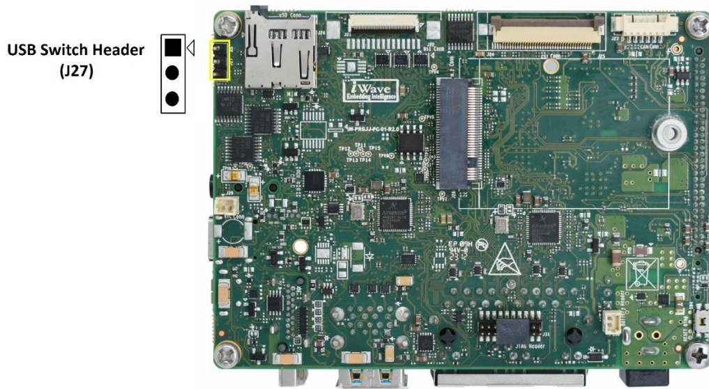
Figure 9: USB Switch Header
