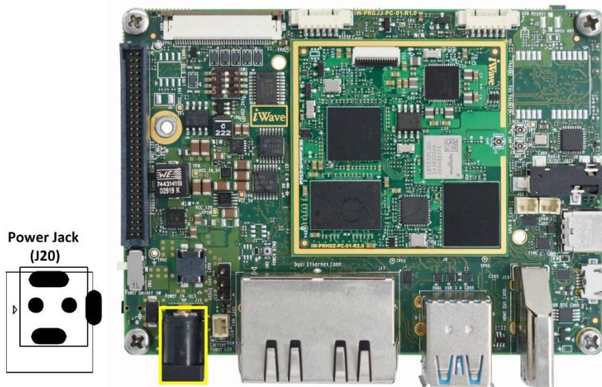
Figure 32: Power Input Jack
