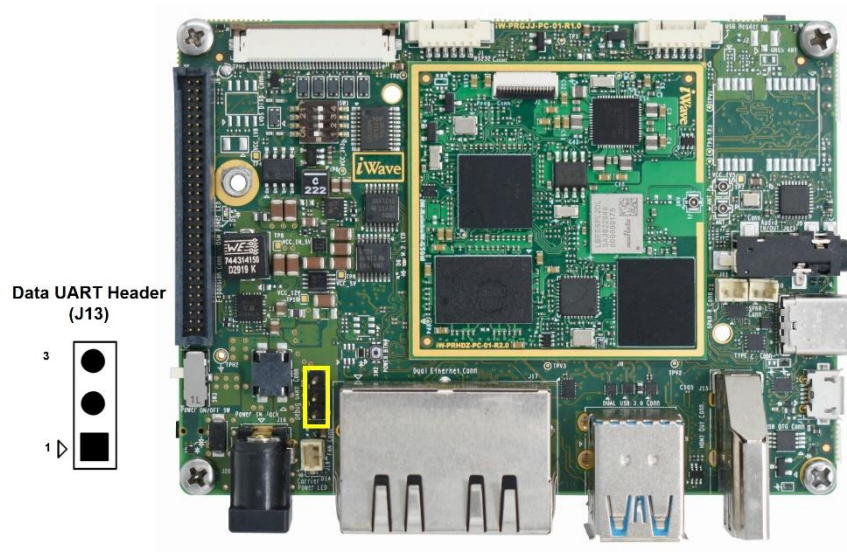
Figure 14: Debug UART Header
