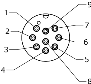
MATING FACE 4282-9PG-300
