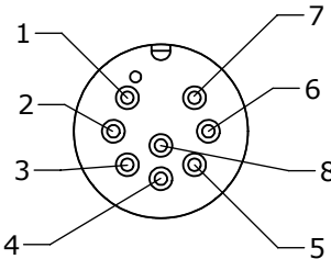
MATING FACE 4282-8PG-300
