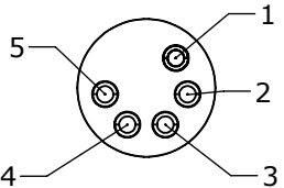
WIRING VIEW 4282-5PG-300
