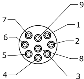
WIRING VIEW 4282-9PG-300
