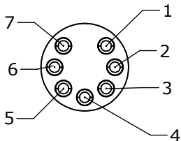
WIRING VIEW 4282-7PG-300
