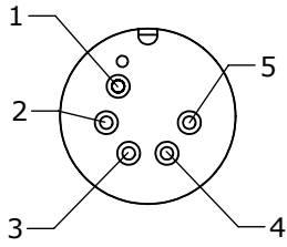
MATING FACE 4282-5PG-300
