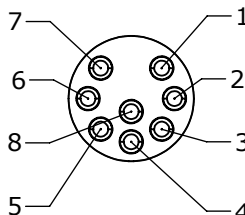
WIRING VIEW 4282-8PG-300
