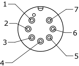
MATING FACE 4282-7PG-300
