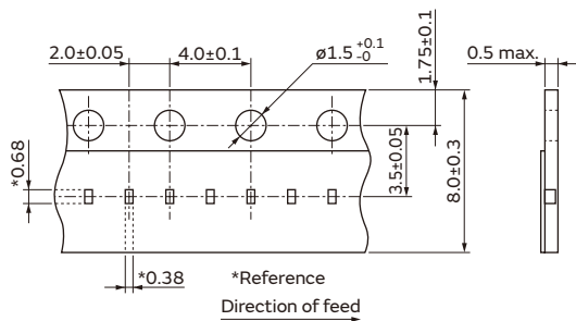
PR*18_RB Series: Paper Tape
