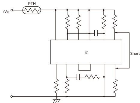
(5) Lock Test of Motor
