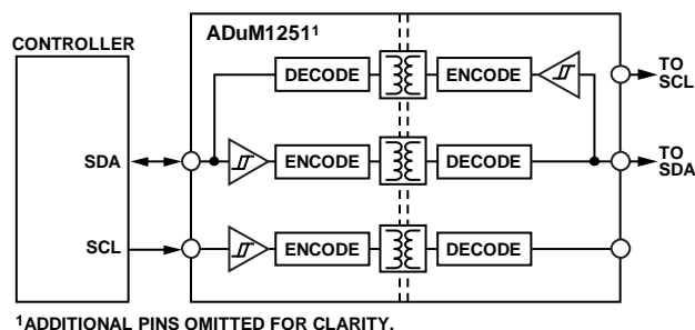
Figure 69. Isolated Interface
