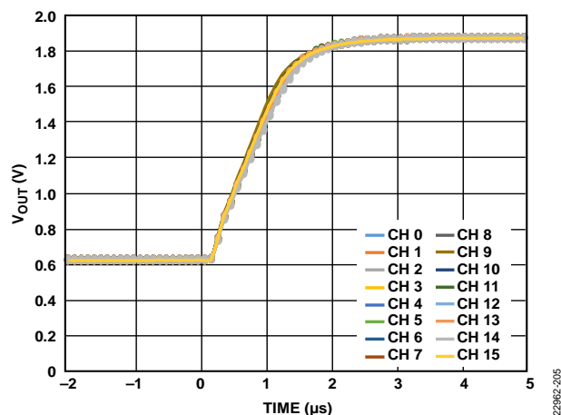
Figure 40. Settling Time
