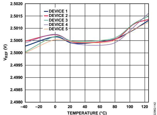
Figure 52. V_{REF} vs. Temperature
