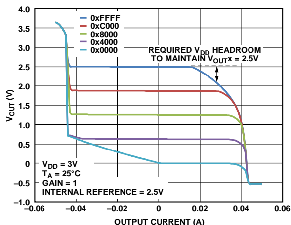
Figure 33. Source and Sink Capability at V_{DD} = 3\text{ V}
