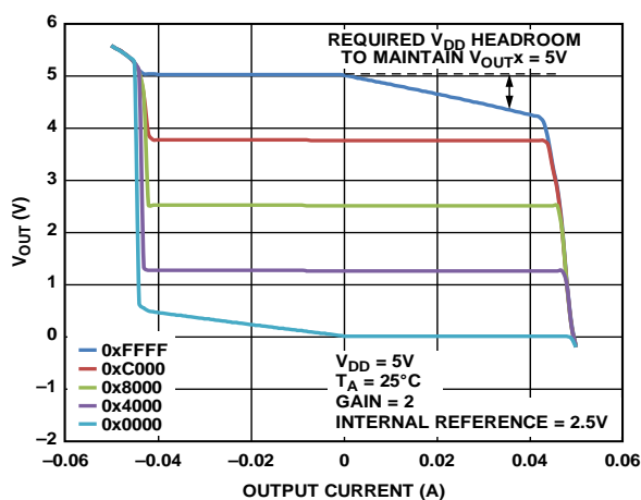
Figure 34. Source and Sink Capability at V_{DD} = 5\text{ V}
