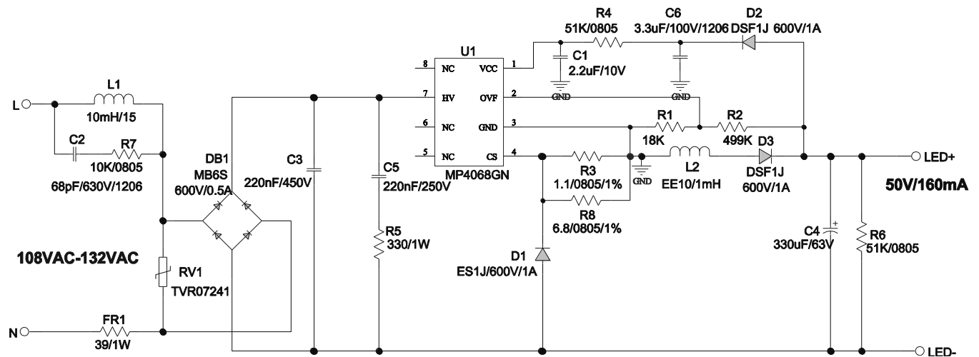
Figure 1—Schematic
