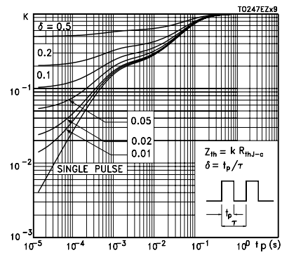
Figure 2. Thermal impedance
