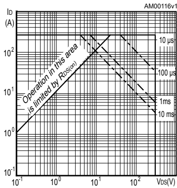
Figure 1. Safe operating area
