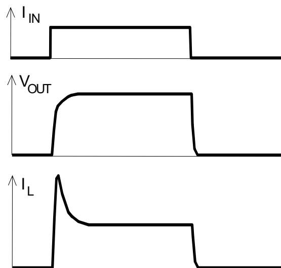
Figure 2b: Switching a lamp
