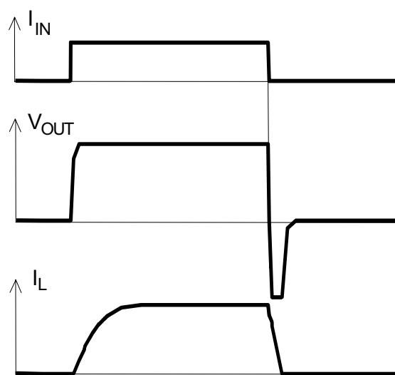
Figure 2c: Switching an inductive load
