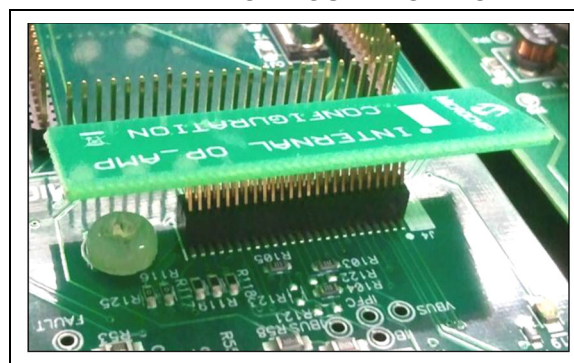
FIGURE 2: INTERNAL OP AMP CONFIGURATION BOARD
