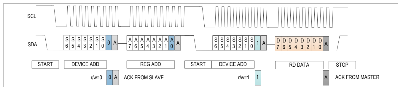
Figure 7. I2C Read
