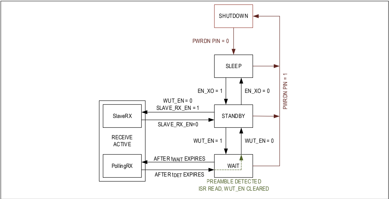
Figure 2. State Diagram
