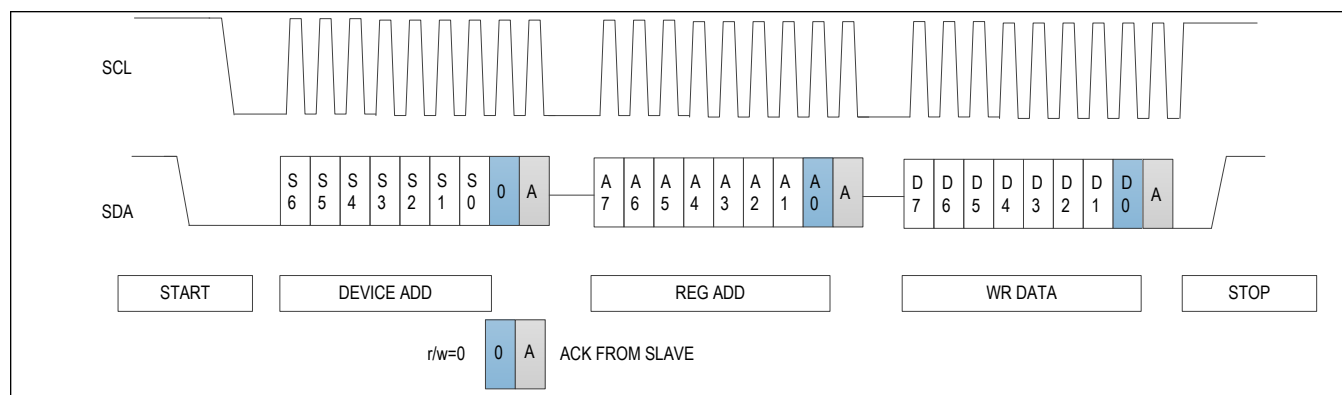
Figure 6. I2C Write
