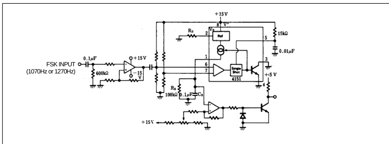
Figure 8. FSK demodulator
