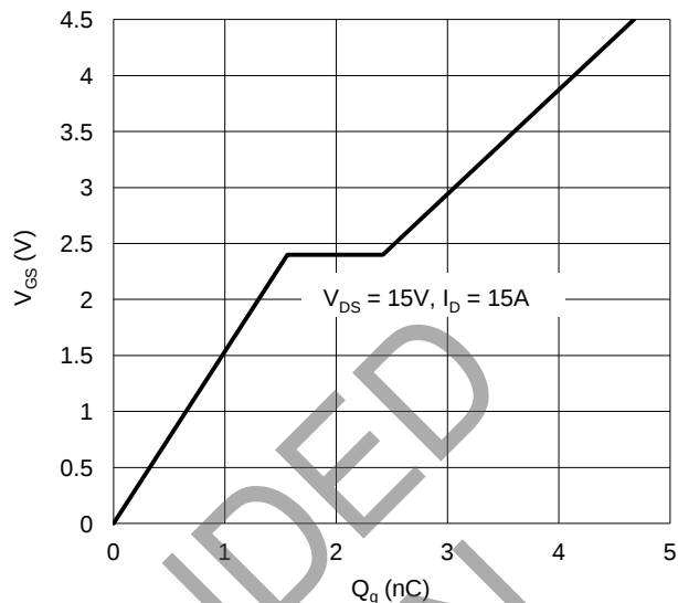
Figure 20. Q2 Gate Charge
