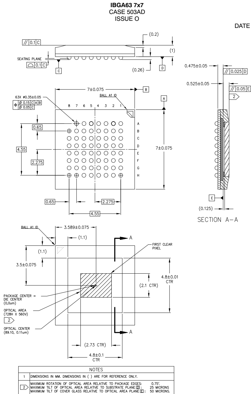
Figure 51: 63-Ball iBGA Package Outline Drawing (Case 503AD)
