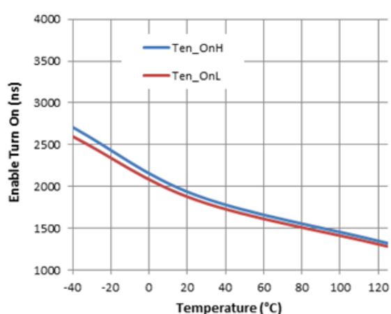
Figure 27. EN to output Ton vs. Temperature
