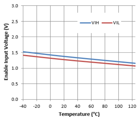
Figure 23. Enable Input Voltage vs. Temperature
