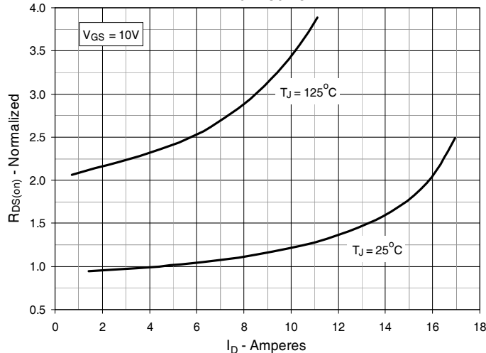
Fig. 5. R_{DS(on)} Normalized to I_D = 4A Value vs. Drain Current
