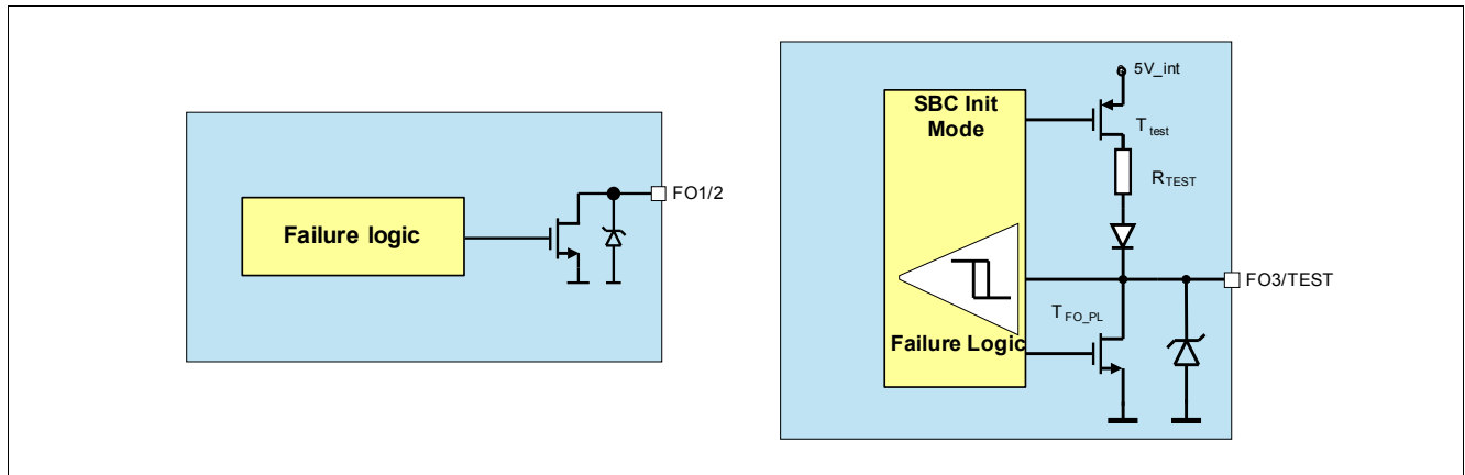
Figure 44 Simplified Fail Output Block Diagram for FO1/2 and for FO3/TEST
