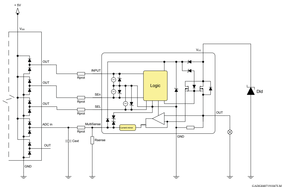
Figure 34. Application diagram
