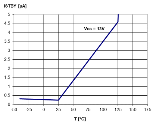
Figure 15. Standby current
