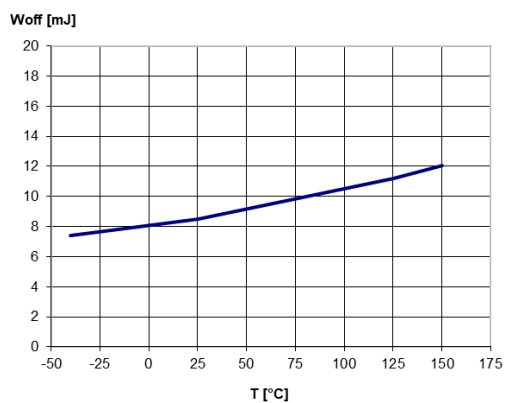
Figure 28. W_{off} vs. T_{case}
