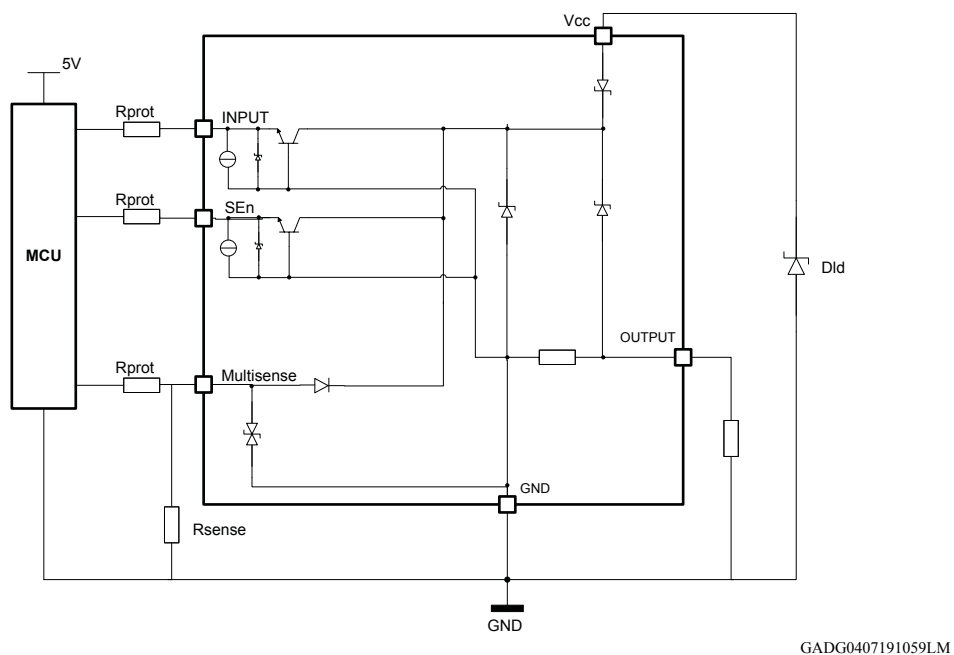
Figure 35. Simplified internal structure
