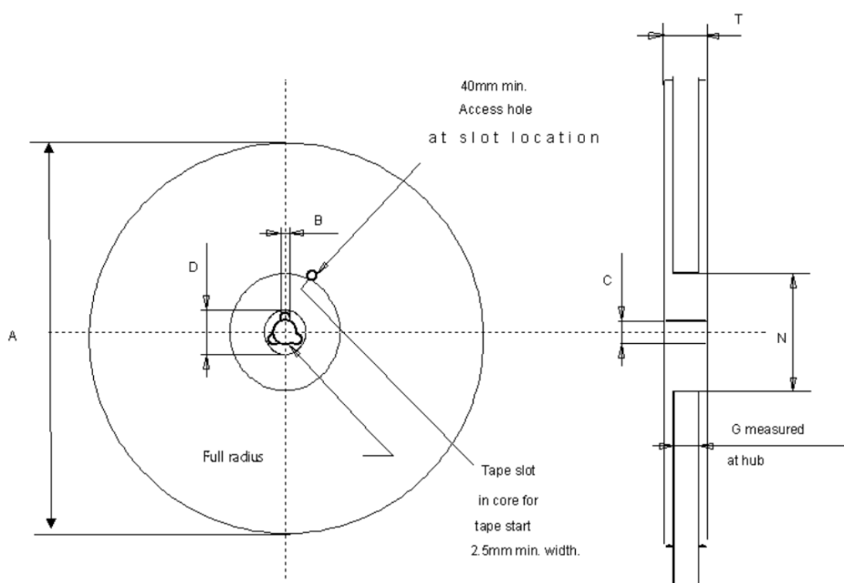
Figure 47. PowerSSO-36 reel 13"
