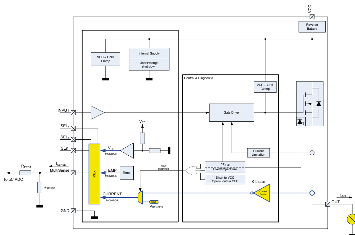
Figure 36. MultiSense and diagnostic – block diagram
