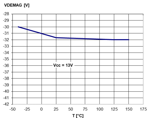
Figure 30. Turn-off output voltage clamp
