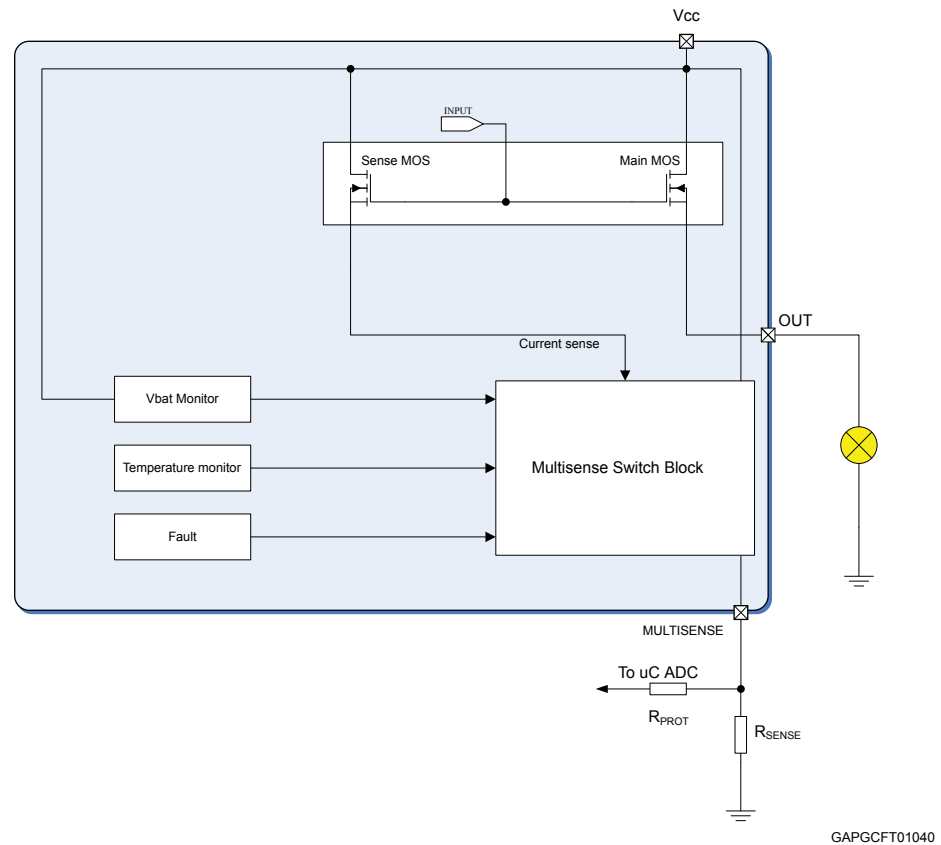
Figure 37. MultiSense block diagram
