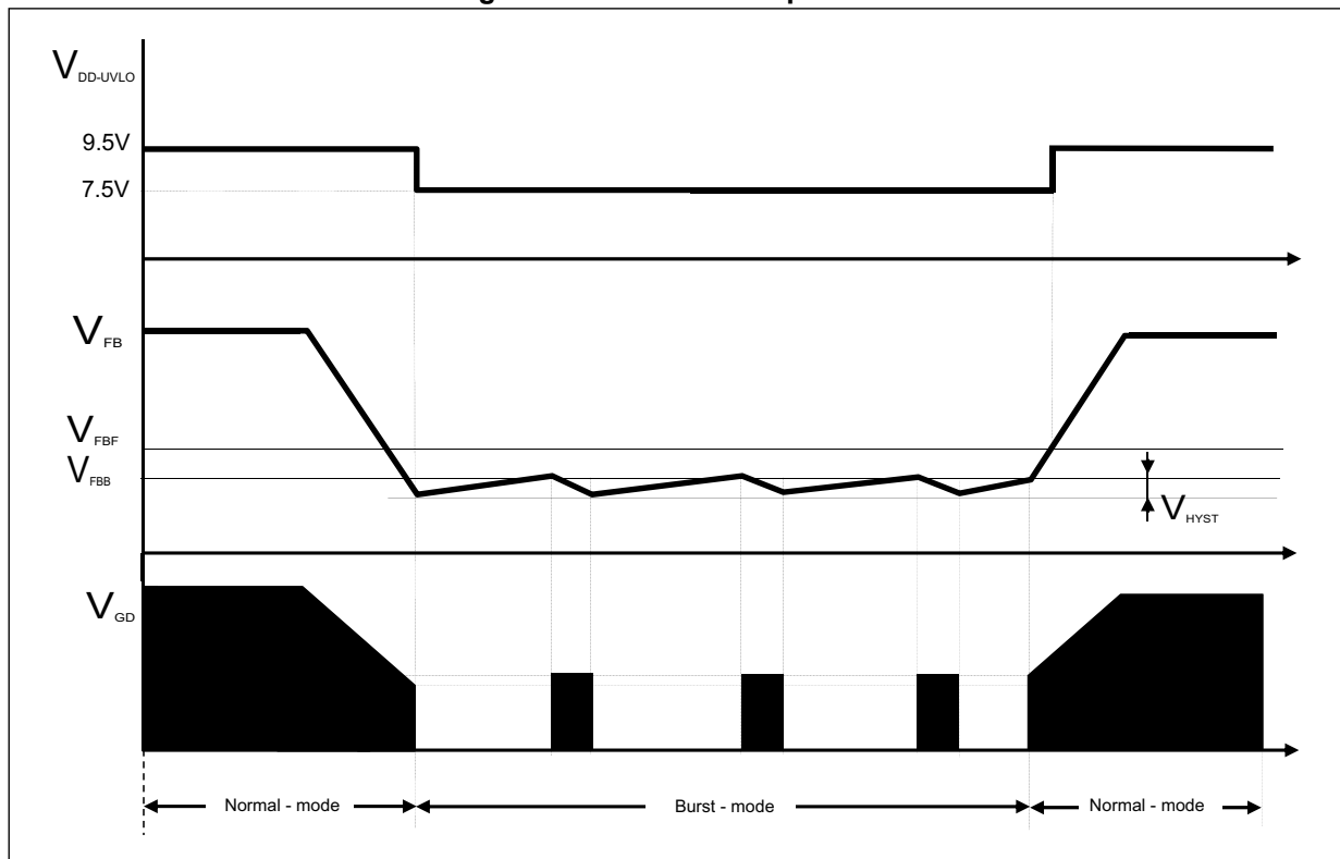
Figure 10. Burst-mode operation
