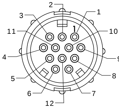
MATING FACE W5280-12PG-5XX
