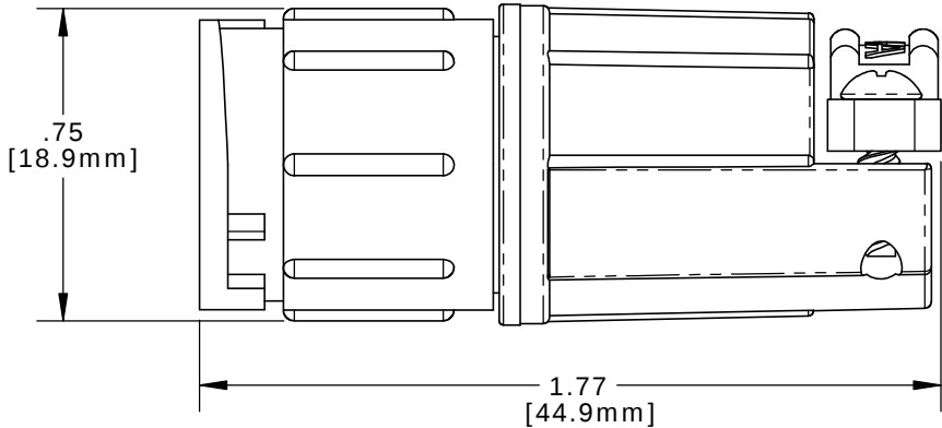
ASSEMBLED VIEW
