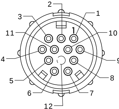
MATING FACE W5280-11PG-5XX
