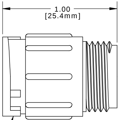
CABLE IN-LINE INSERT, MALE MAT'L: UV THERMOPLASTIC, BLACK
