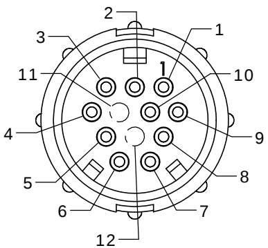
MATING FACE W5280-10PG-5XX
