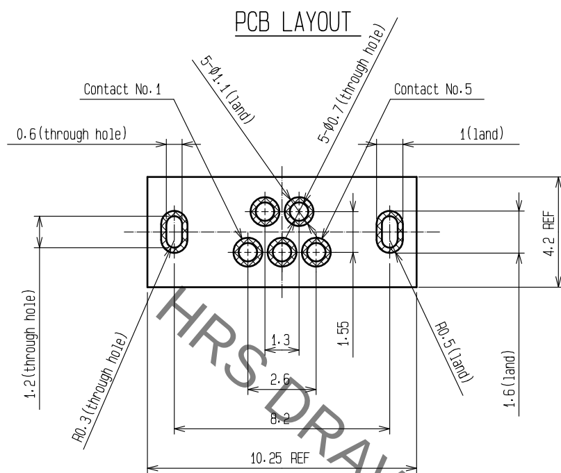
ZX20-B-SLDC
