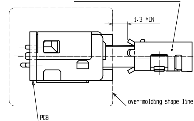
ZX SERIES RECEPTACLE
