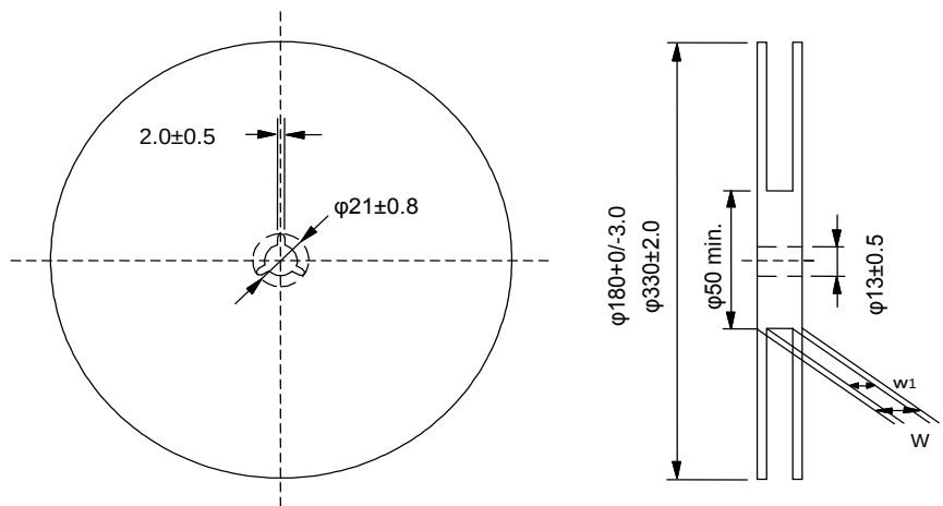
Fig.3 Taping Diagram
