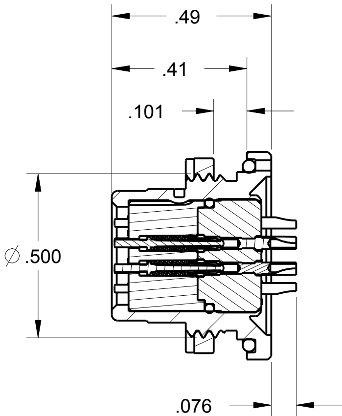
SECTION Z-Z
