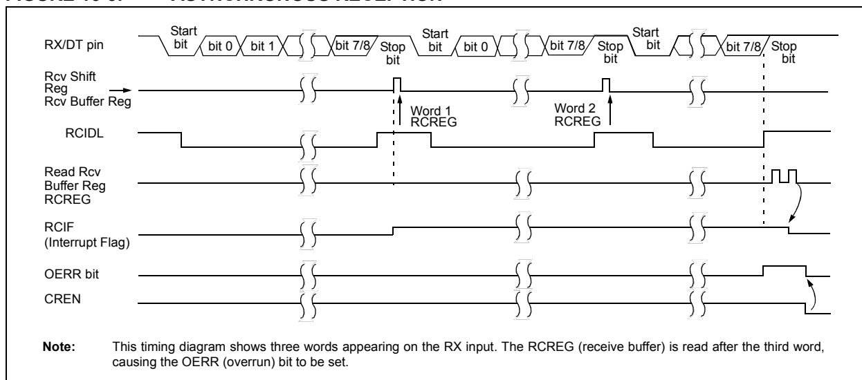
FIGURE 16-5: ASYNCHRONOUS RECEPTION
