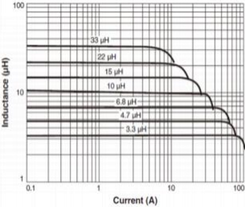
LvsCurrent
