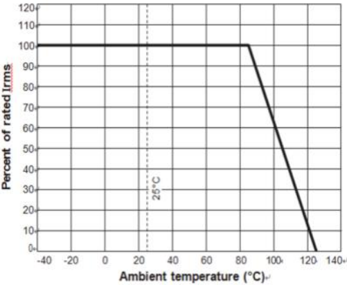
Irms Derating
