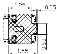
RECOMMENDED PCB LAYOUT TOLERANCE:±0.05MM (FOR REFERENCE ONLY)
