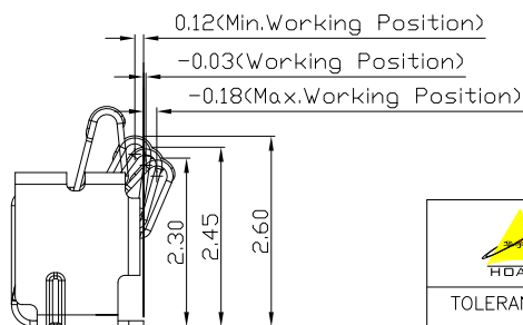
(For Reference Only) Stated At Compression
