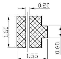
METAL MASK T=0.08 TOLERANCE:±0.05MM (FOR REFERENCE ONLY)
