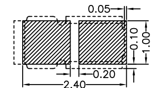
RECOMMENDED PCB LAYOUT TOLERANCE: ±0.05
