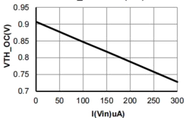
VTH_OC vs. I(Vin)
