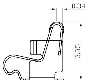
(For Reference Only) Stated At Compression
