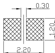
METAL MASK T=0.08 TOLERANCE:±0.05MM (FOR REFERENCE ONLY)
