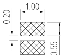
METAL MASK T=0.08 TOLERANCE: ±0.05MM (FOR REFERENCE ONLY)
