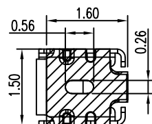
RECOMMENDED PCB LAYOUT TOLERANCE ±0.05 (焊盘推荐图)
