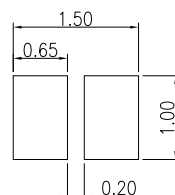
METAL MASK T=0.10 TOLERANCE±0.05 (钢网推荐图)
