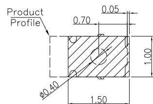
RECOMMENDED PCB LAYOUT TOLERANCE±0.05 (焊盘推荐图)
