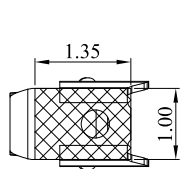
RECOMMENDED PCB LAYOUT TOLERANCE:±0.05MM (FOR REFERENCE ONLY)
