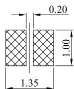
METAL MASK T=0.08 TOLERANCE:±0.05MM (FOR REFERENCE ONLY)
