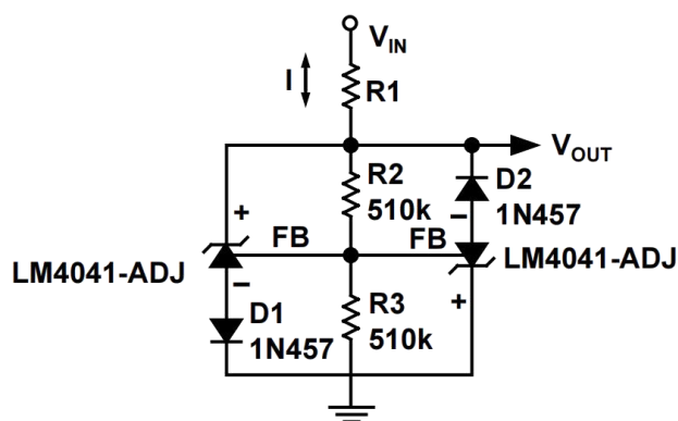
Figure 6. Bidirectional Clamp +2.4V
