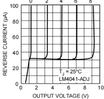
Reverse Characteristics †
