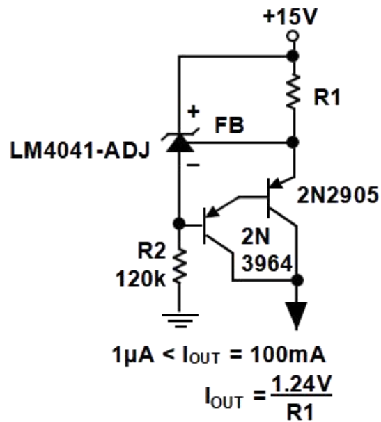
Figure 10. Current Source
