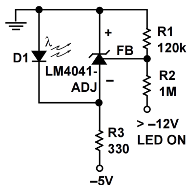
Figure 4. Voltage Level Detector
