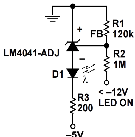
Figure 3. Voltage Level Detector
